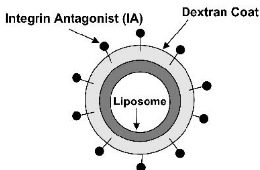
Fig. 1. Structure of integrin antagonist and representation of an IA-DCL.
