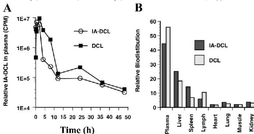
Fig. 2. (A) Plasma clearance of ^{14}\text{C} -labeled IA-DCLs and DCLs lacking IA in nu/nu mice. (B) Biodistribution of IA-DCLs and DCLs in healthy mice at 24 h. For these studies, IA-DCL and DCL were injected intravenously and plasma or tissue samples were pooled. The standard deviation was less than 10% for repeat measurements of a given sample.
